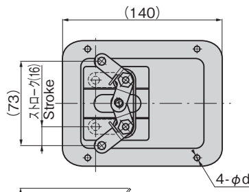
[A-1880-1W] 2点締めタイプ 2-point securing type
