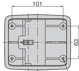
4-φ4.2深さ11 depth M5タッピンねじ用下穴 hole for tap
