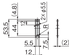
〔調整板〕Adjusting plate
