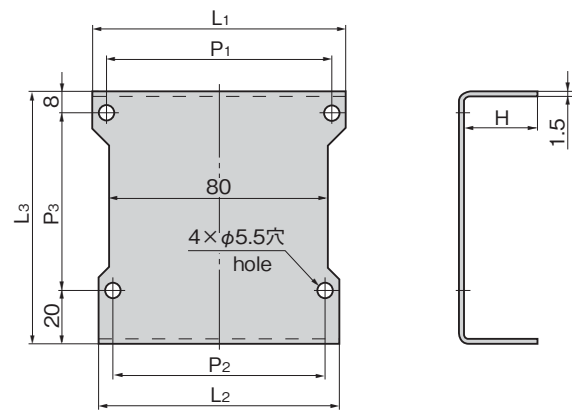
[A-873-1-P] [A-873-2-P] 取付け板 Installation plate
