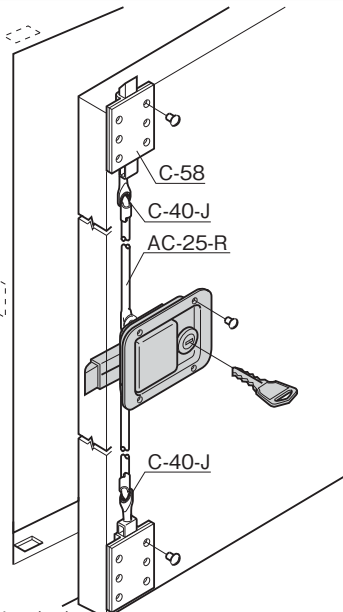
3点締め 3-point securing lock
