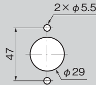
止め金 Stopper plate
