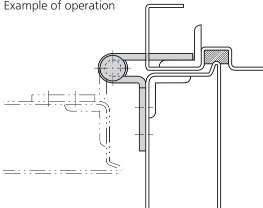
作動例 Example of operation
