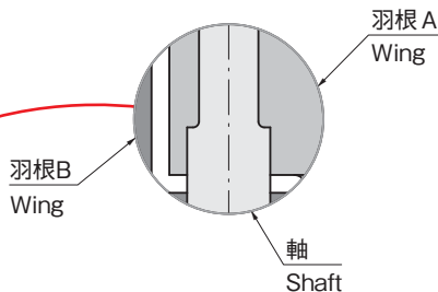
摺動部断面 Sliding side cross section
