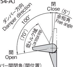
ダンパー開閉角(開位置) Damper open/close angles (closed position)
