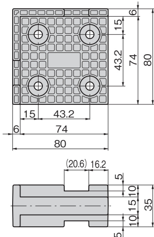
CP-660-B (爪付きタイプ) (With catch)
