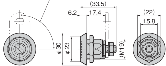
止め金回転角度90° Stopper plate turning angle (33.5)
