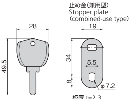
板厚 t=2.3 Plate thickness
