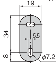
板厚 t=2.3 Plate thickness
