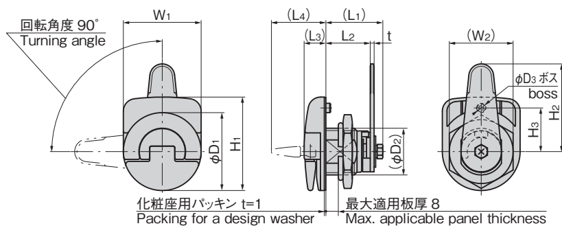
〔本体/化粧座あり〕 Main body / With a design washer
