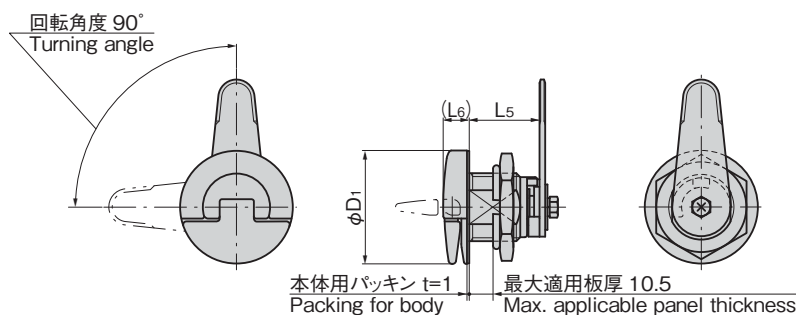
〔本体/化粧座無し〕 Main body / Without a design washer
