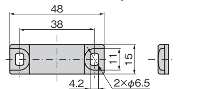
C-185-B [本体 Main body]
