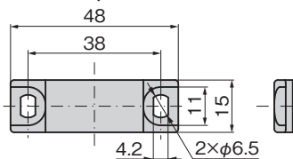
[受板 Catch plate]
