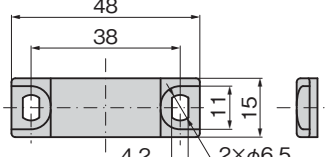
[受板 Catch plate]
