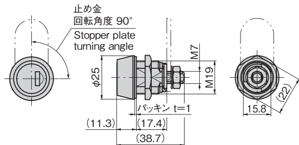
止め金(兼用型) Stopper plate (combined-use type)
