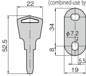
板厚 t=2.3 Plate thickness
