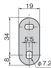
板厚 t=2.3 Plate thickness
