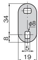
板厚 t=3.2 Plate thickness
