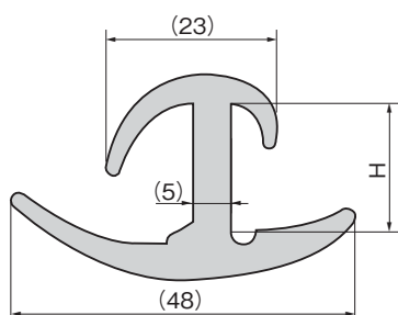
〔FC-784〕保冷車用ゴム 長さ2.5m Rubber for cold storage vehicle
