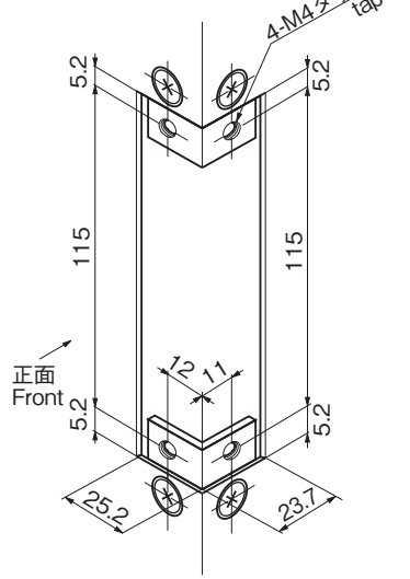
取付け穴加工例 Example of machining installing holes
