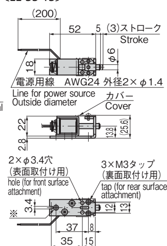
[LE-33-13]
