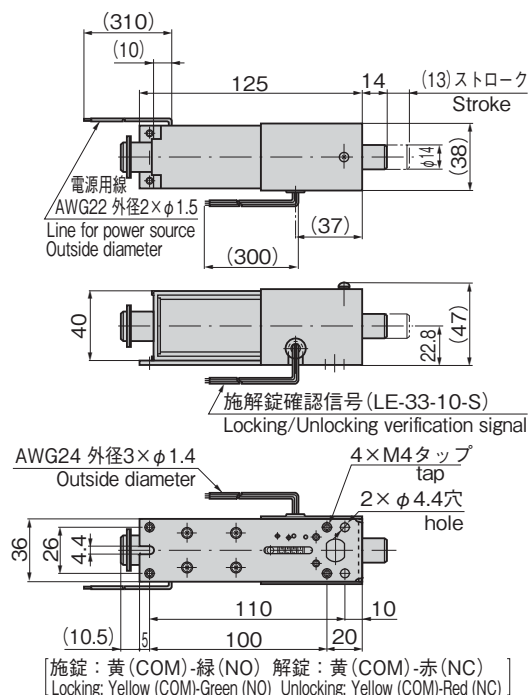
[LE-33-10・LE-33-10-S]
