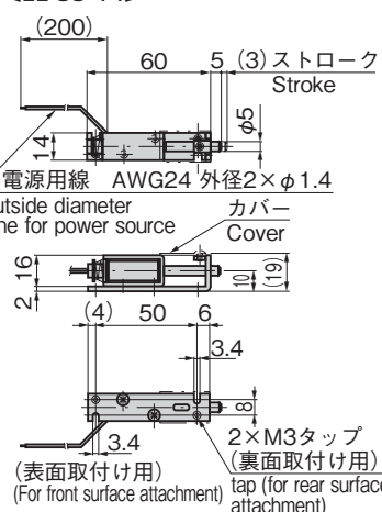
[LE-33-14]
