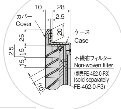
A部断面 Cross-section of A
